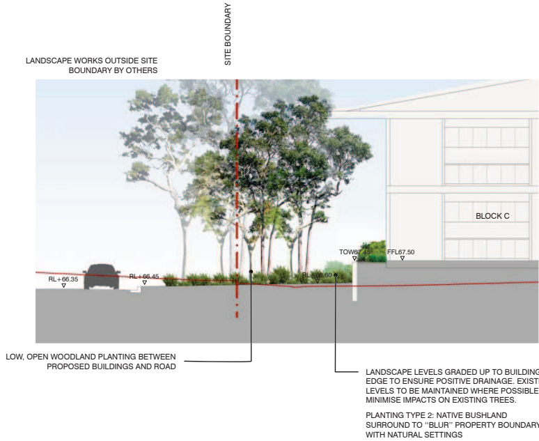
SECTION THROUGH COMMUNAL AREA
