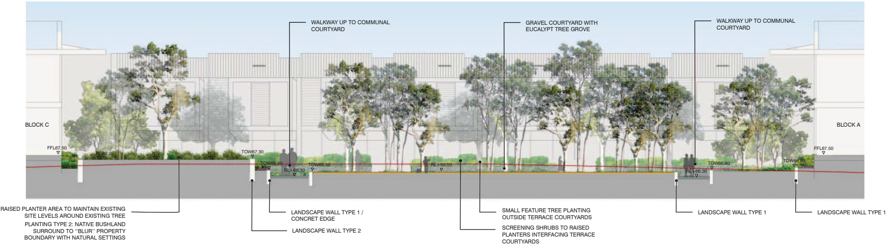
SECTION THROUGH COMMUNAL AREA
